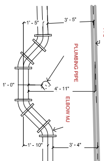
2 UNDERGROUND SECTION VIEW #2
