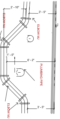
3 UNDERGROUND SECTION VIEW #3
